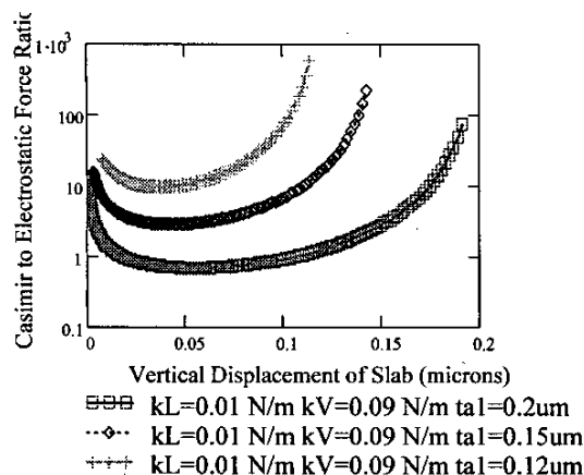
Figure 6. Ratio of Casimir force to electrostatic as a function of top and bottom air-gap asymmetry about dielectric slab. Parameters: \epsilon_d=7.5 , \epsilon_a=1 , t_d=1.1\mu\text{m} , t_d=0.6\mu\text{m} , t_{a2}+t_{a2}=0.5\mu\text{m} .
