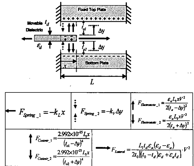
Figure 2. Forces acting on dielectric slab.
